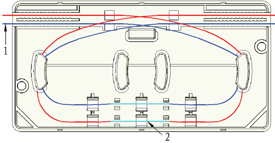
1 - Fiber optic cable 2 - Heat protection shrinkable sleeve
