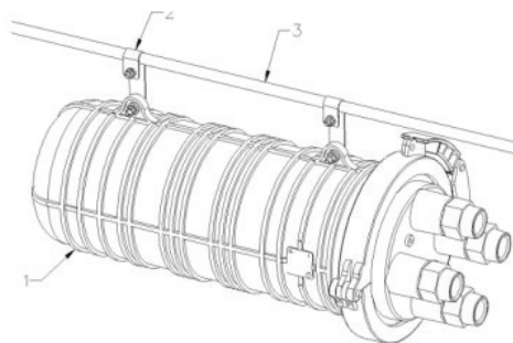
1— closure 2-- Aerial hanged accessory 3— steel wire
